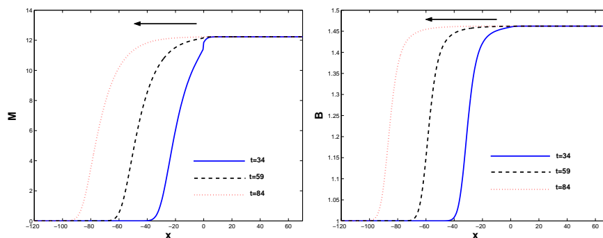
FIGURE 7. Wave profiles for mistletoes (left) and birds (right) of the traveling wave solution of (2) for the kernel defined by (37) with \sigma = 2 and other parameters given in Table 1.
