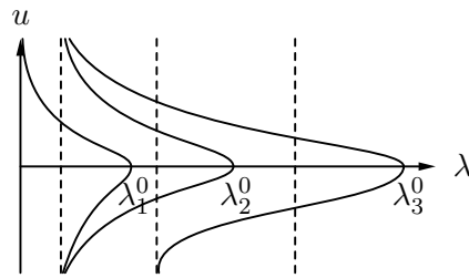
Figure 2: Bifurcation from \infty for (1, \infty) -type f
