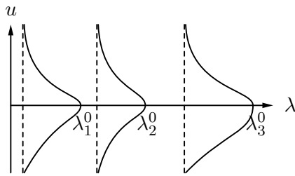
Figure 1: Bifurcation from \infty for (1, 1) -type f
