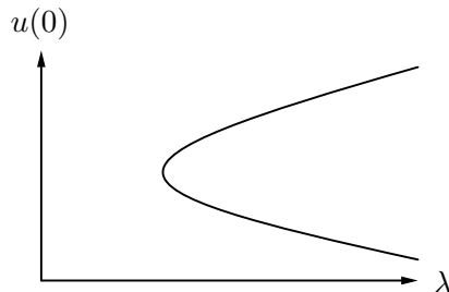
Figure 4: Theorem 4
