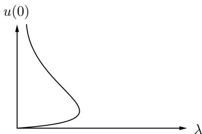
Figure 1: Theorem 1
