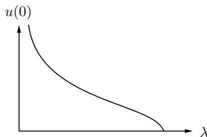
Figure 2: Theorem 2
